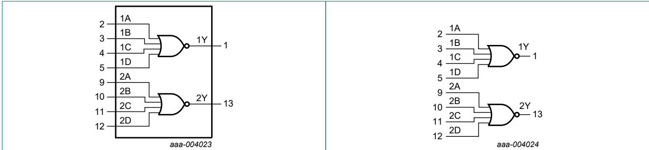
Fig. 1. Functional diagram
