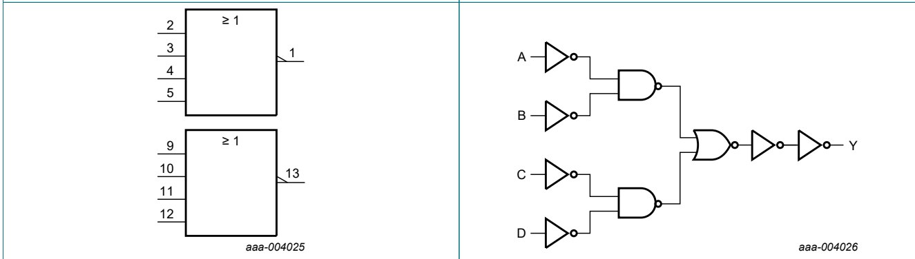
Fig. 3. IEC Logic symbol
